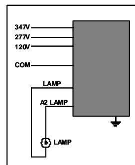
Wiring Diagram
