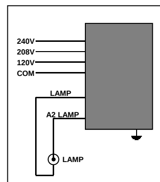
Wiring Diagram
