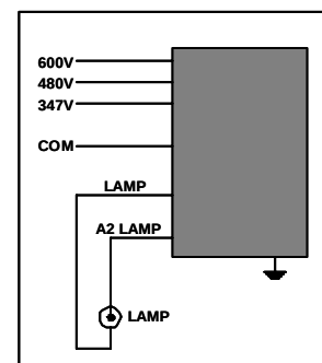
Wiring Diagram
